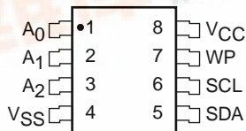
SOIC Package (J, K, W, X)
