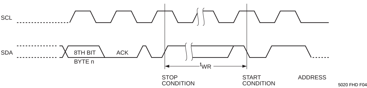
Figure 3. Start/Stop Timing
