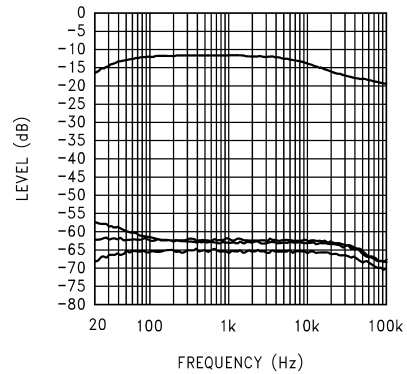
Top Trace = No Cap, Next Trace Down = 1\mu f Next Trace Down = 2\mu f , Bottom Trace = 4.7\mu f
