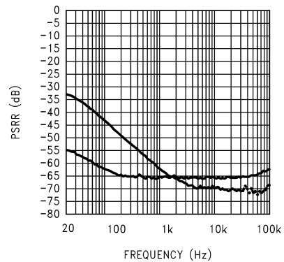
HWD2190 = Bottom Trace HWD2177 = Top Trace
