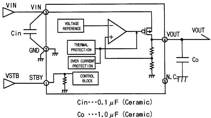
Fig.1 BLOCK DIAGRAM and APPLICATION CIRCUIT
