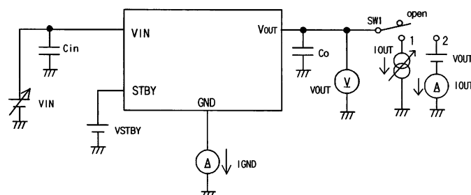
Fig.2 TEST CIRCUIT
