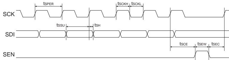
Figure 24: Detailed Timing Diagram for Serial Interface
