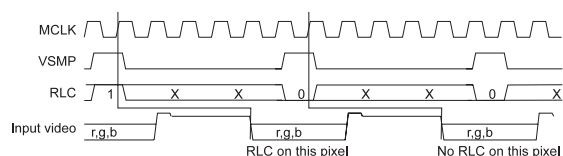
Figure 6: RLC Timing
