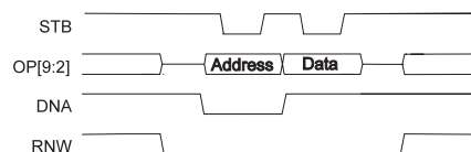
Figure 17: Parallel Interface Timing
