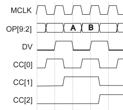
Figure 11: Eight-bit Multiplexed Bus Output
