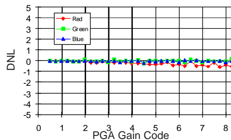
PGA DNL @ MCLK = 8MHz
