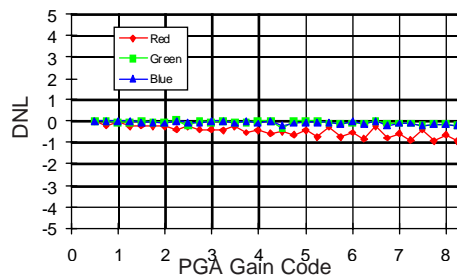
PGA DNL @ MCLK = 12.3MHz
