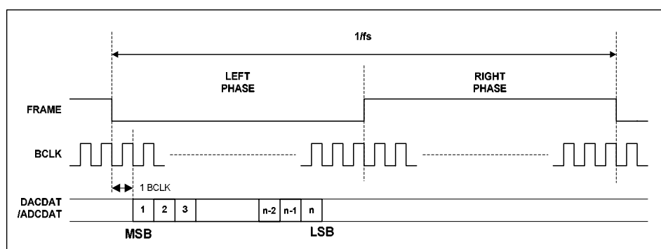
Figure 22 I 2 S Audio Interface (assuming n-bit word length)
