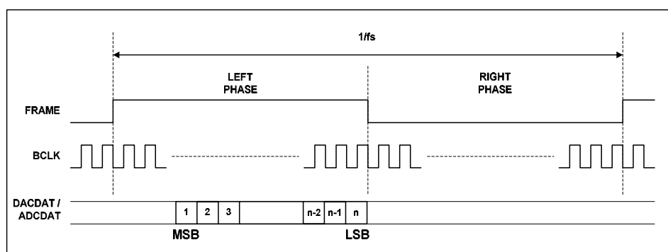
Figure 21 Right Justified Audio Interface (assuming n-bit word length)
