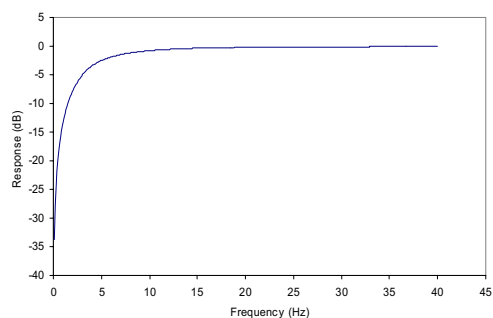
Figure 40 ADC Highpass Filter Response, HPFAPP=0
