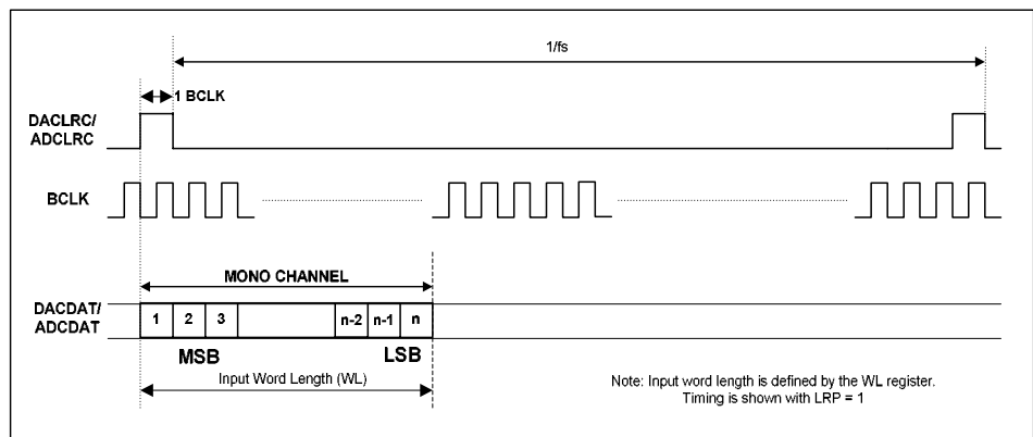
Figure 17 DSP Mode Audio Interface (mode B, LRP=1)
