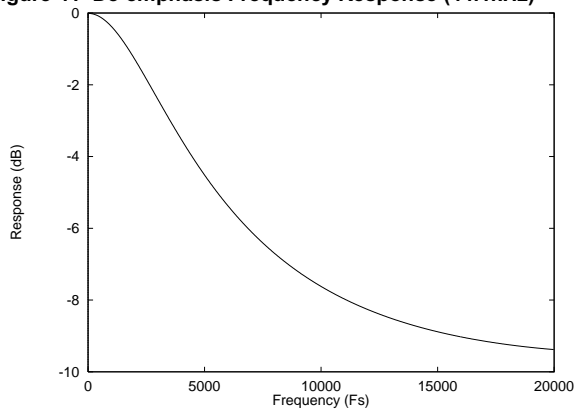
Figure 43 De-emphasis Frequency Response (48kHz)
