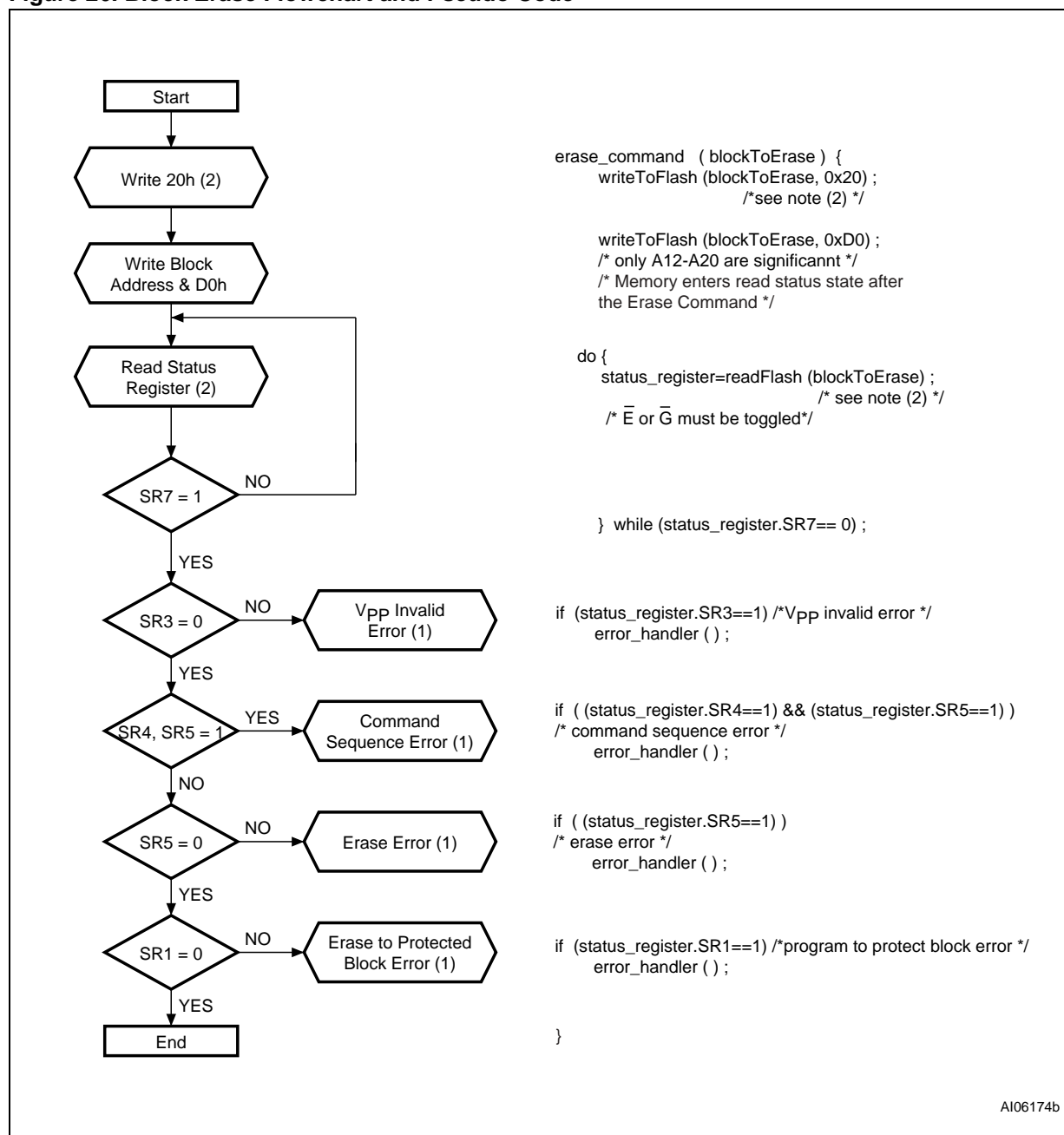
Figure 26. Block Erase Flowchart and Pseudo Code
