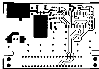
Figure 12. COMP Side
