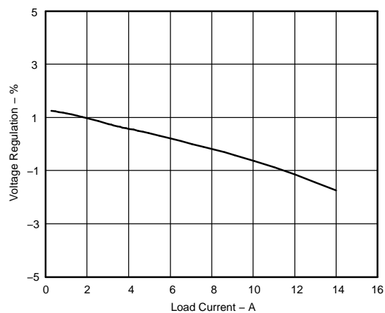
Figure 19. Load Regulation
