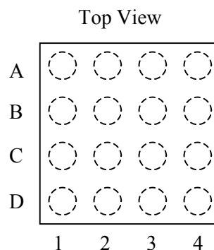
16-Ball STPBGA (4mm x 4mm) 14-Pin Flip Chip (100-mil x 100-mil) (Not Shown)
