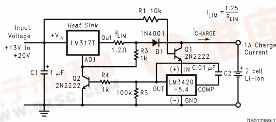
Typical Constant Current/Constant Voltage Li-Ion Battery Charger
