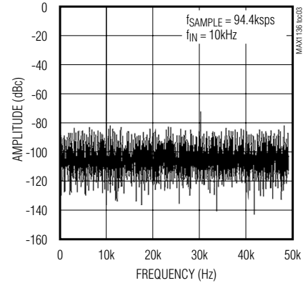
FFT PLOT
