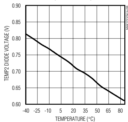
TEMP2 DIODE VOLTAGE vs. TEMPERATURE
