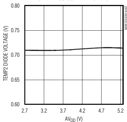
TEMP2 DIODE VOLTAGE vs. ANALOG SUPPLY VOLTAGE
