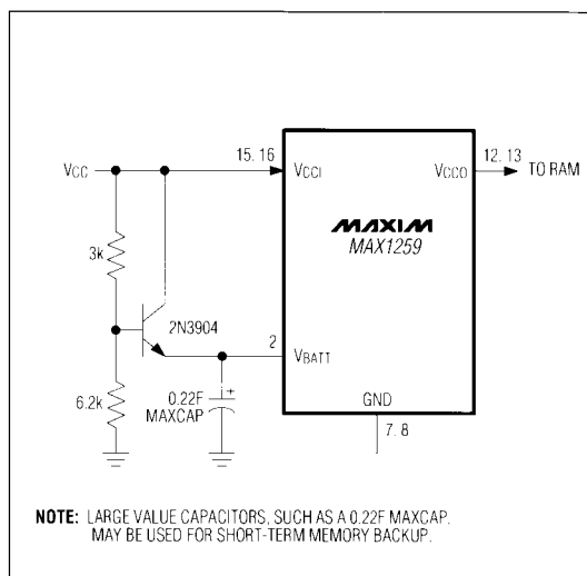
Figure 3. Using a MAXCAP as a Backup Battery
