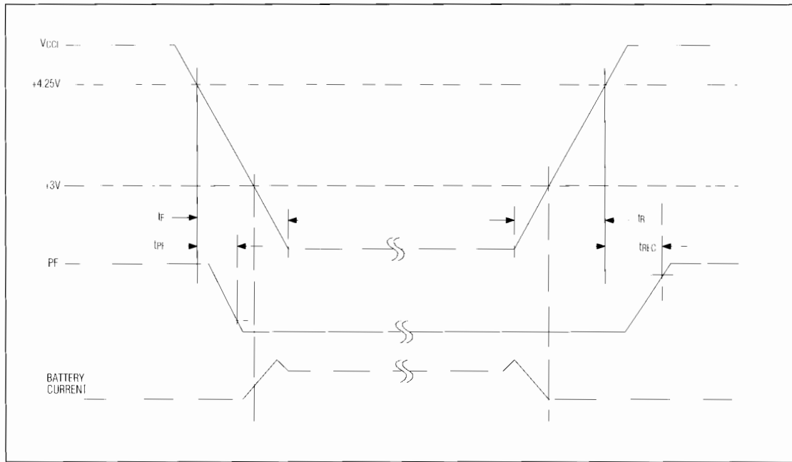
Figure 1. Power-Down/Power-Up Conditions
