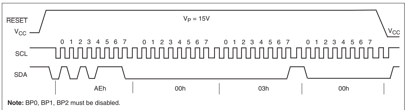
Figure 7. Reset V_{TRIP} Level Sequence
