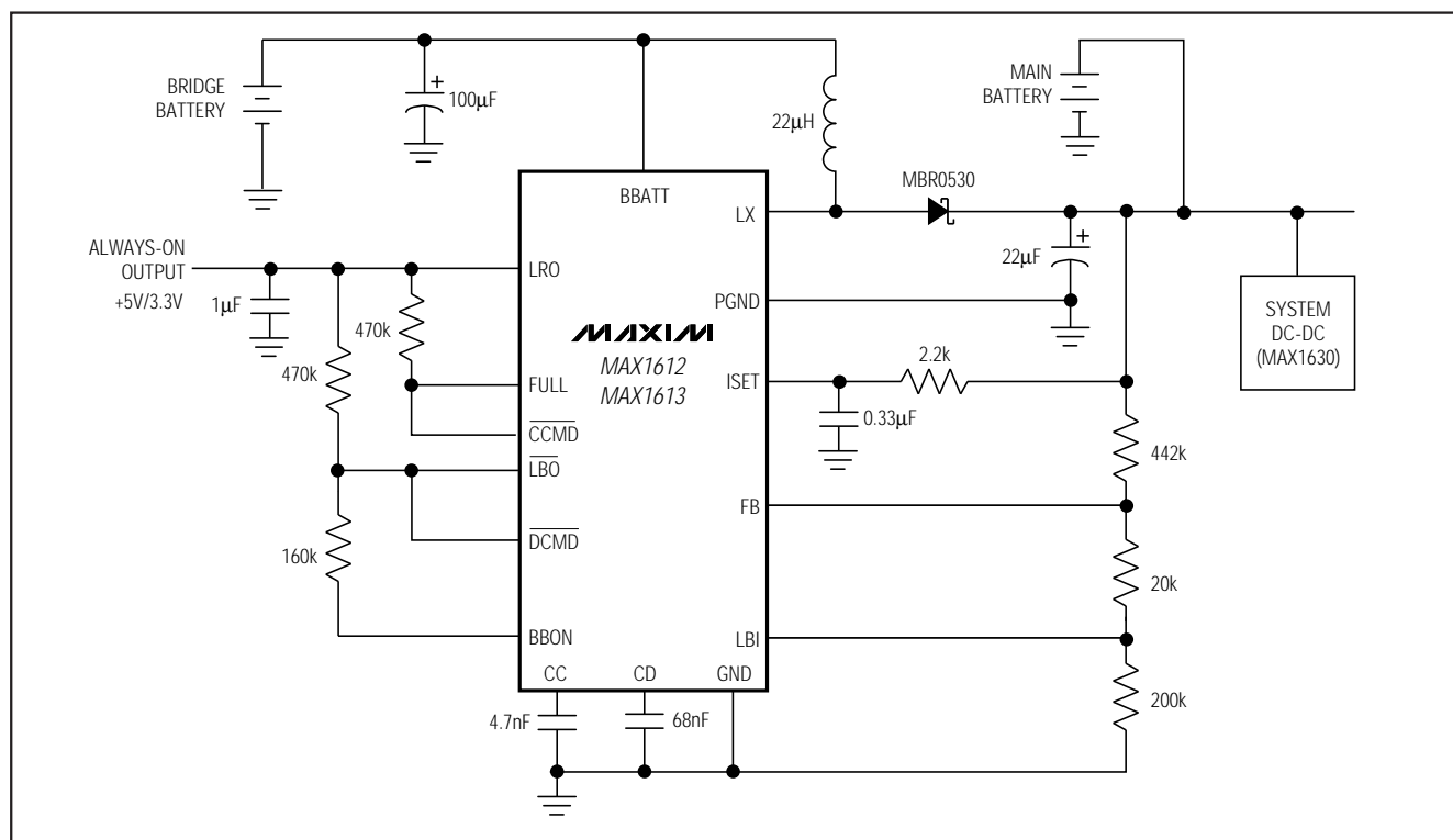
Figure 3. Stand-Alone Application
