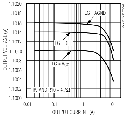
MAX1624 OUTPUT VOLTAGE vs. OUTPUT CURRENT ( V_{OUT} = 1.1\text{V} )
