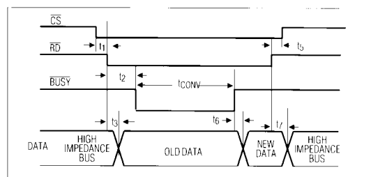
Figure 3. Slow-Memory Interface Mode Timing Diagram
