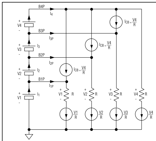
Figure 4. Cell Voltage Sampling
