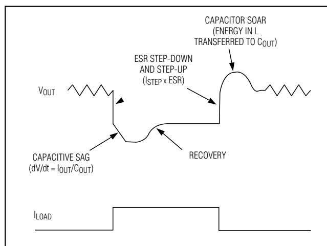
Figure 10. Transient-Response Regions
