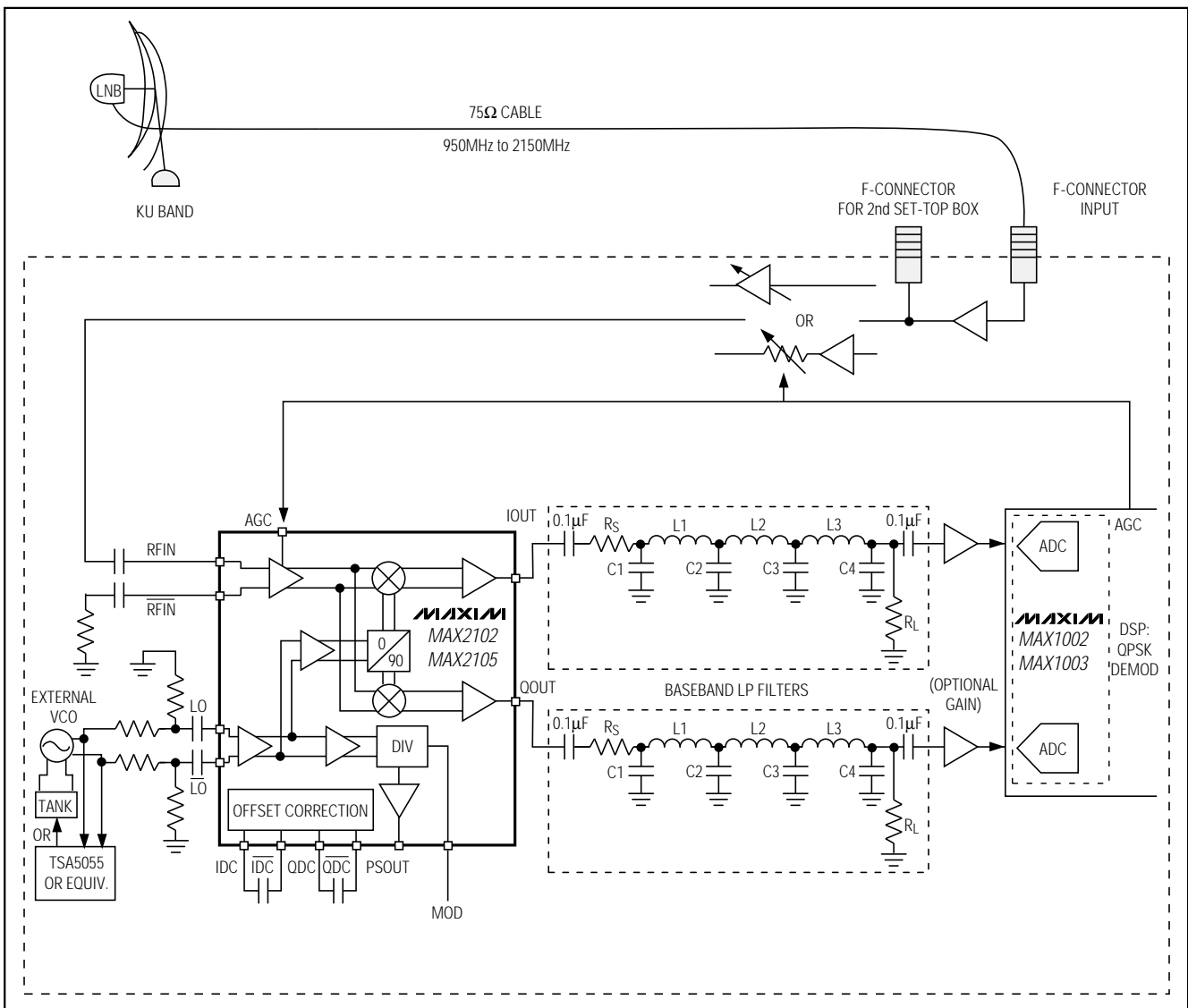
Figure 2. Typical Application
