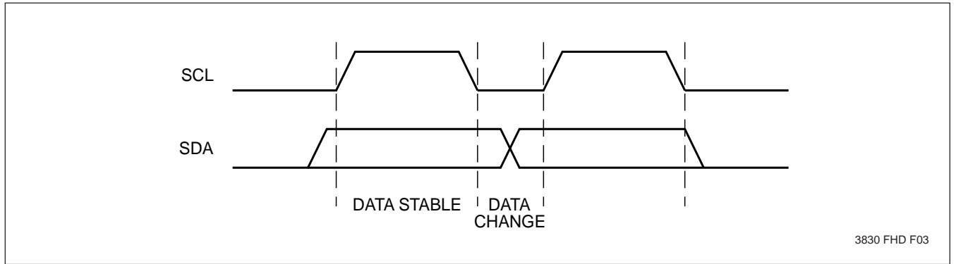
Figure 1. Data Validity
