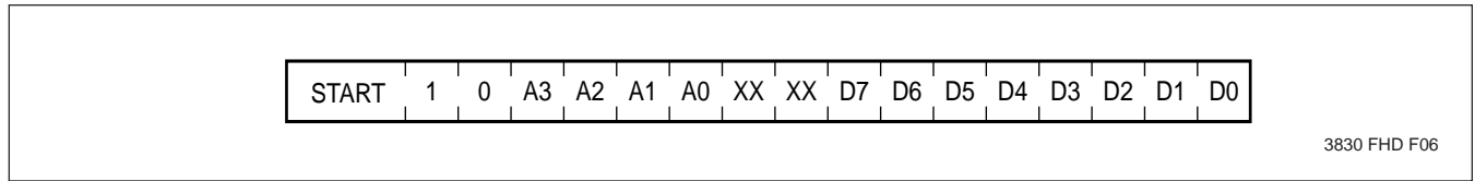
Figure 4. Read Sequence
