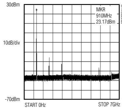
SPURIOUS LEVEL FROM DC TO 7TH HARMONIC
