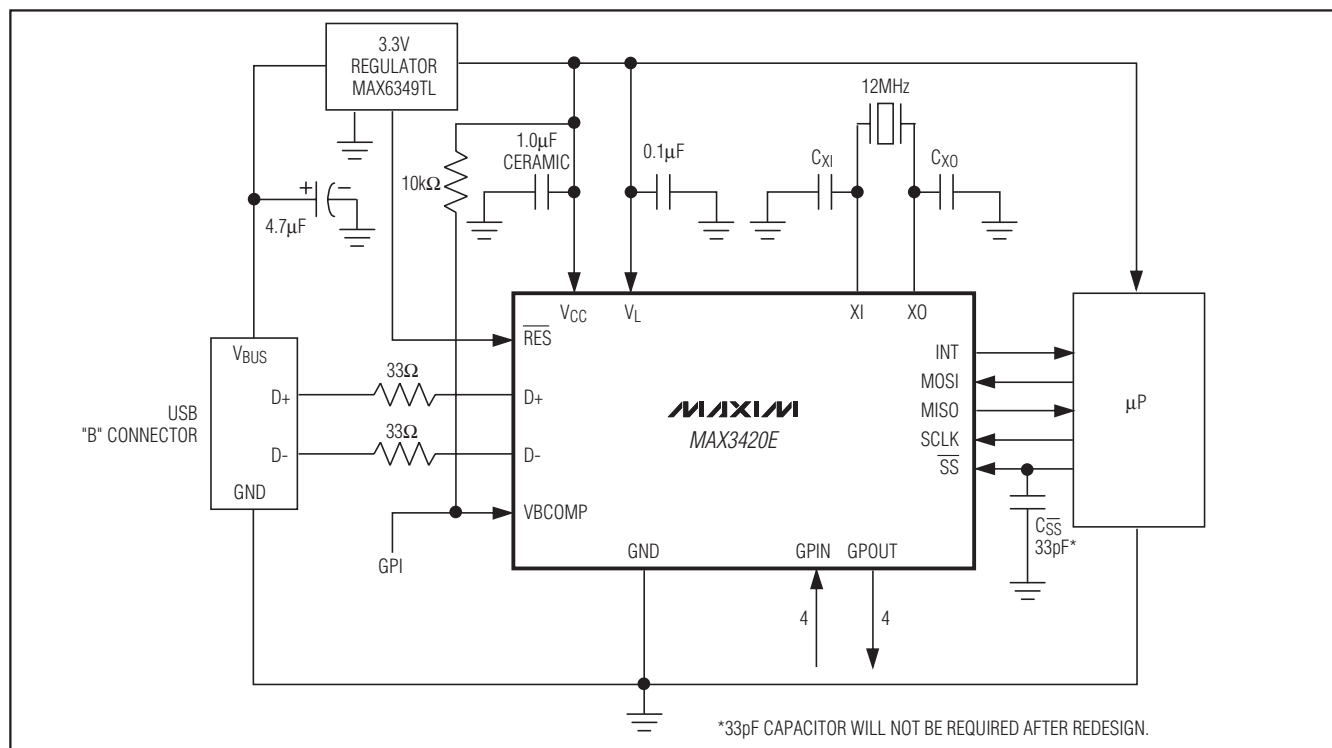
Figure 16. MAX3420E in a Bus-Powered Application
