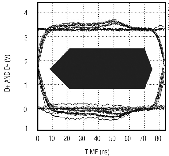
EYE DIAGRAM
