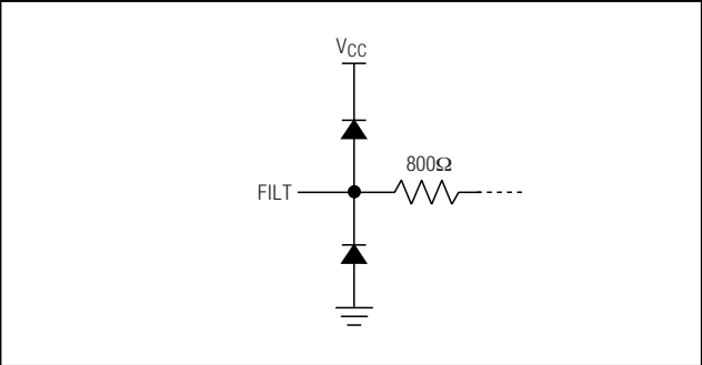
Figure 7. FILT Interface
