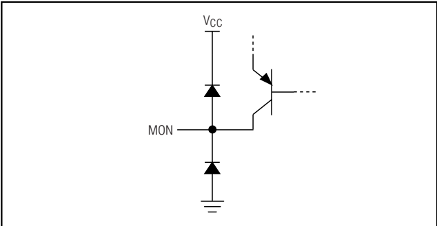
Figure 8. MON Interface
