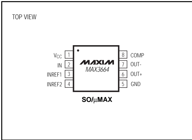
Pin Configuration
