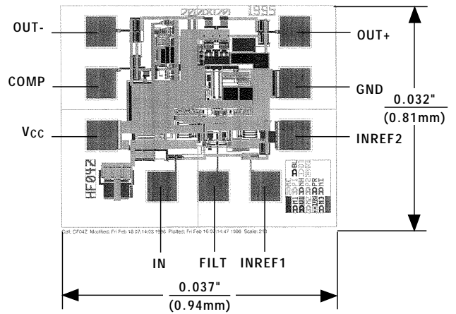
Chip Topography
