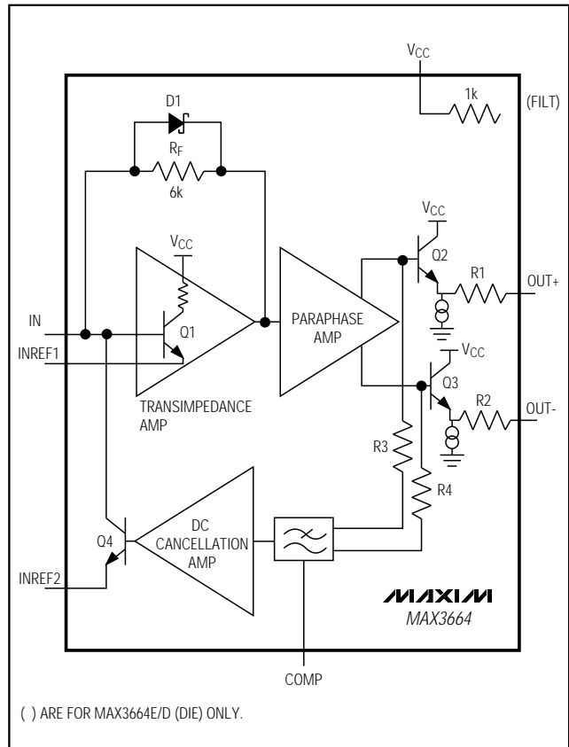
Figure 1. Functional Diagram
