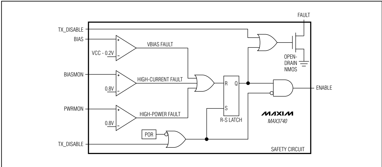
Figure 2. Safety Circuit
