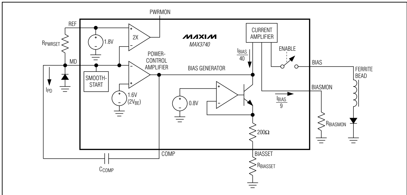
Figure 1. Bias Generator
