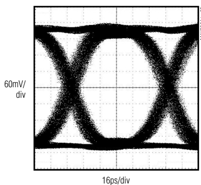
EQUALIZER OUTPUT EYE AFTER 18in OF FR-4 (27PRBS WITH 100 CIDs AT 10.7Gbps)
