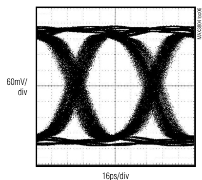
EQUALIZER OUTPUT EYE AFTER 18in OF FR-4 (K28.5 AT 12.5Gbps)
