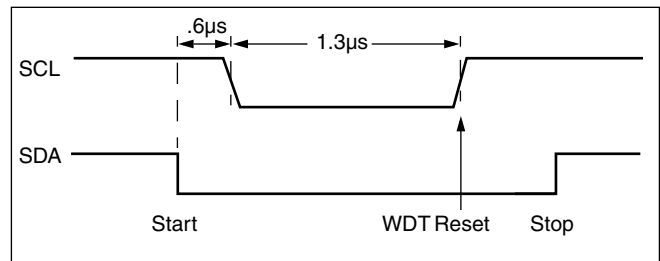
Figure 1. Watchdog Restart
