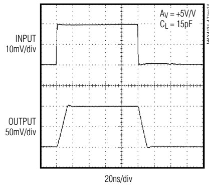
MAX4435/MAX4437 SMALL-SIGNAL PULSE RESPONSE
