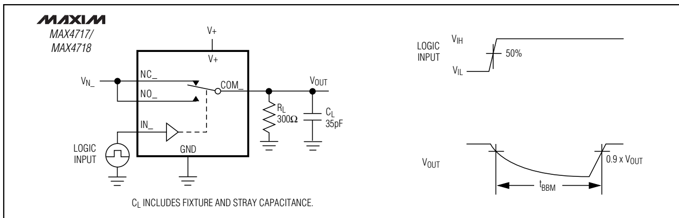
Figure 2. Break-Before-Make Interval
