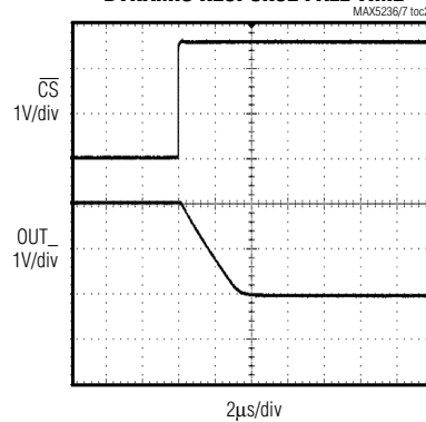
MAX5236 DYNAMIC RESPONSE FALL TIME
