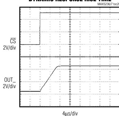
MAX5237 DYNAMIC RESPONSE RISE TIME
