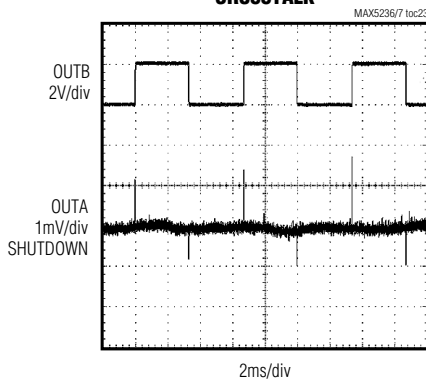
MAX5236 CROSSTALK
