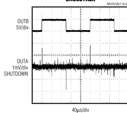
MAX5237 CROSSTALK
