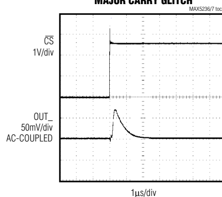
MAX5236 MAJOR CARRY GLITCH
