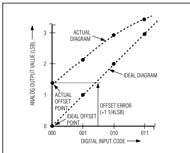
Figure 6c. Offset Error
