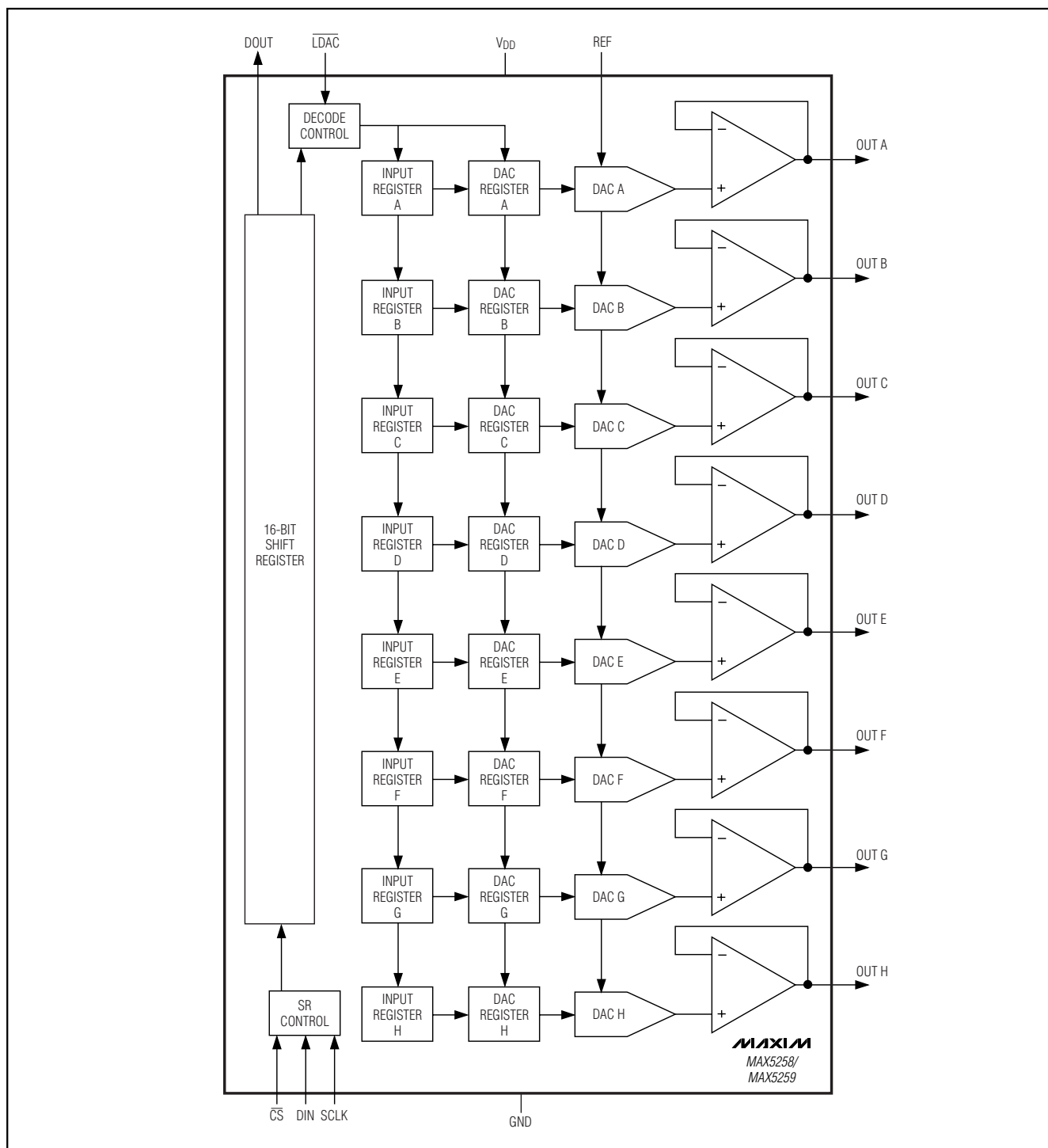
Functional Diagram
