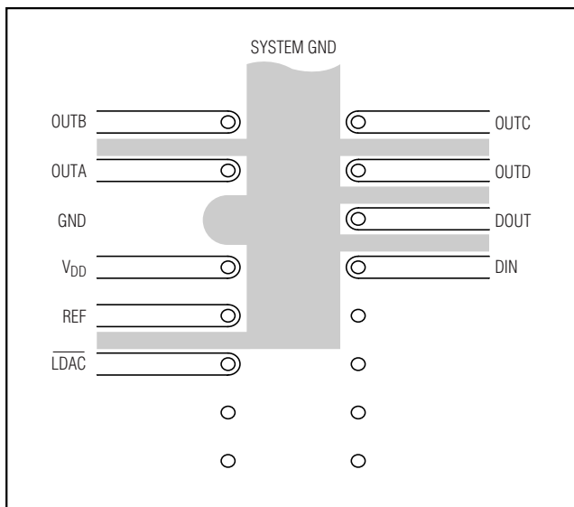
Figure 10. Suggested PC Board Layout for Minimizing Crosstalk (Bottom View)
