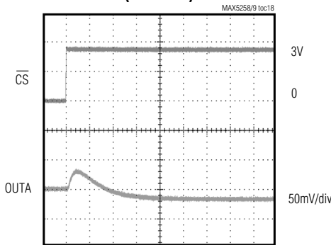
WORST-CASE 1LSB DIGITAL STEP CHANGE (NEGATIVE)
