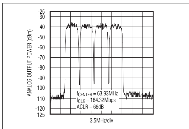
Figure 10. ACLR for W-CDMA Modulation, Four Carriers
