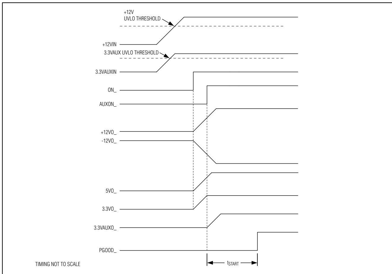
Figure 1. Startup Waveforms
