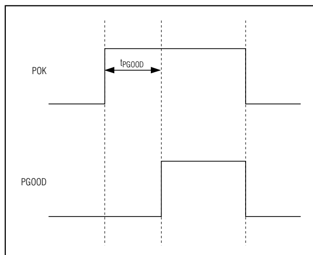
Figure 3. PGOOD Timing
