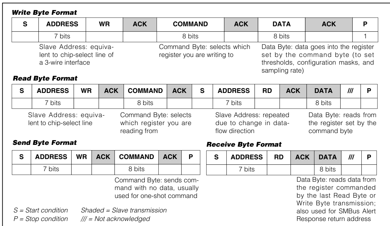
Figure 1. SMBus Protocols
