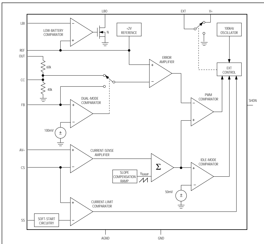
Figure 2. Block Diagram
