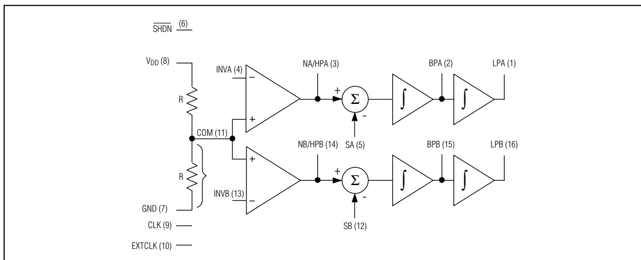
Figure 1. Block Diagram
