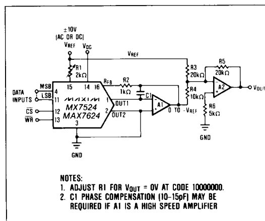
Figure 4. Bipolar (4-Quadrant) Operation
