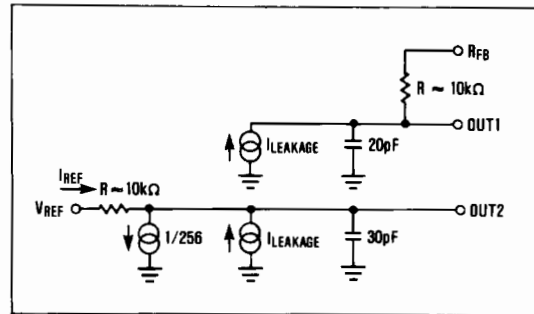
Figure 2. MX7524/MAX7624 DAC Equivalent Circuit—All Digital Inputs LOW
