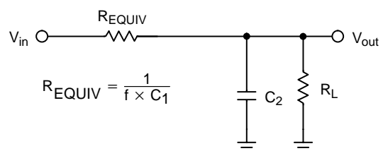
Figure 23. Equivalent Output Resistance
