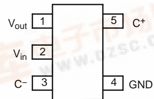
Thin SOT-23-5* (Top View)
