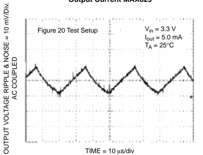
Figure 19. Output Voltage Ripple and Noise MAX829
