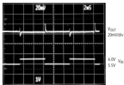
LINE-TRANSIENT RESPONSE
