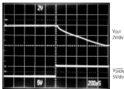
MAX850/MAX851/MAX853 START-UP FROM SHUTDOWN
