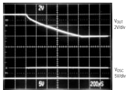
MAX852 START-UP FROM SHUTDOWN
