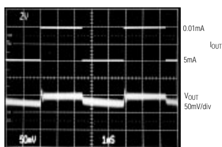
LOAD-TRANSIENT RESPONSE
