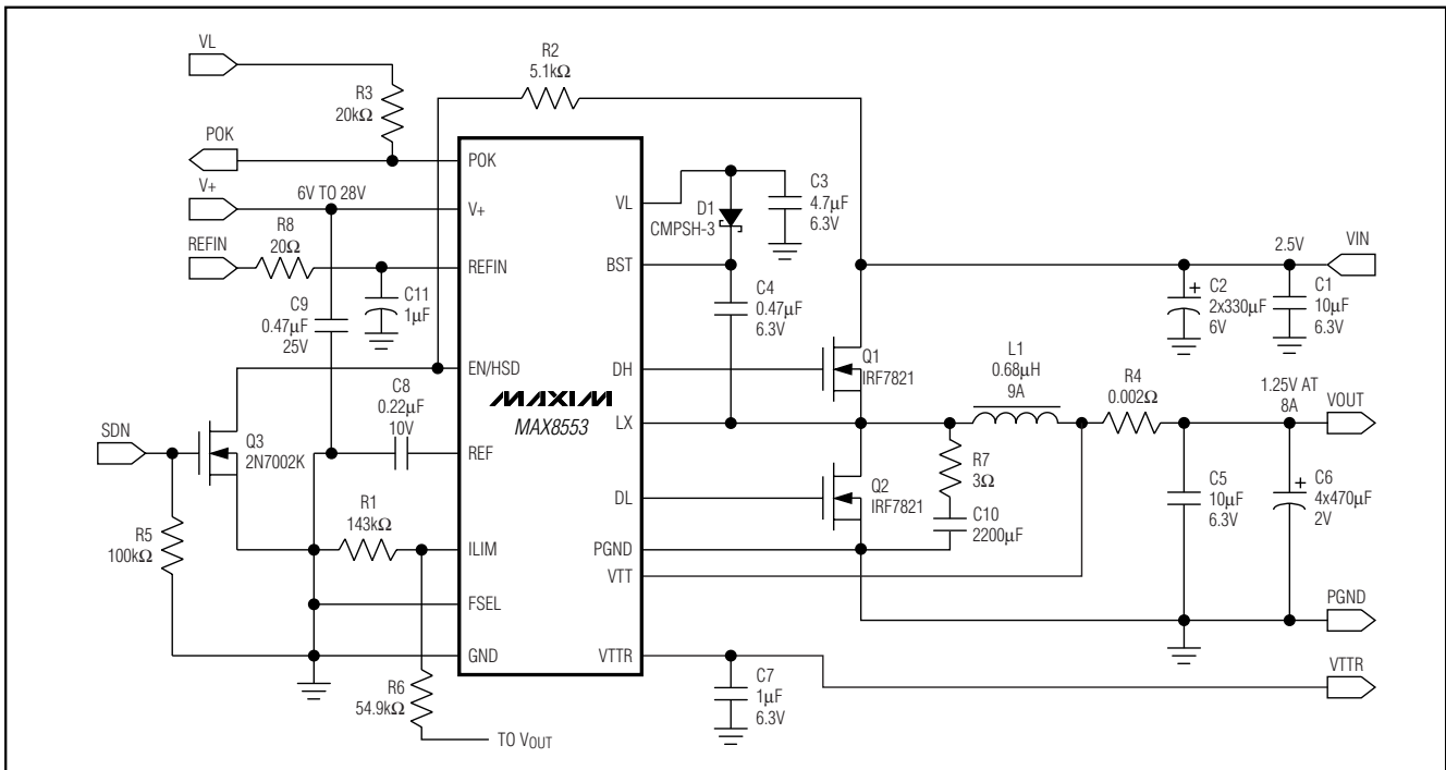
Figure 2. Typical Application Circuit 2: 2.5V Input, 1.25V VTT at Up to 8A, and 1.25V VTT at Up to 25mA with 550kHz Switching
