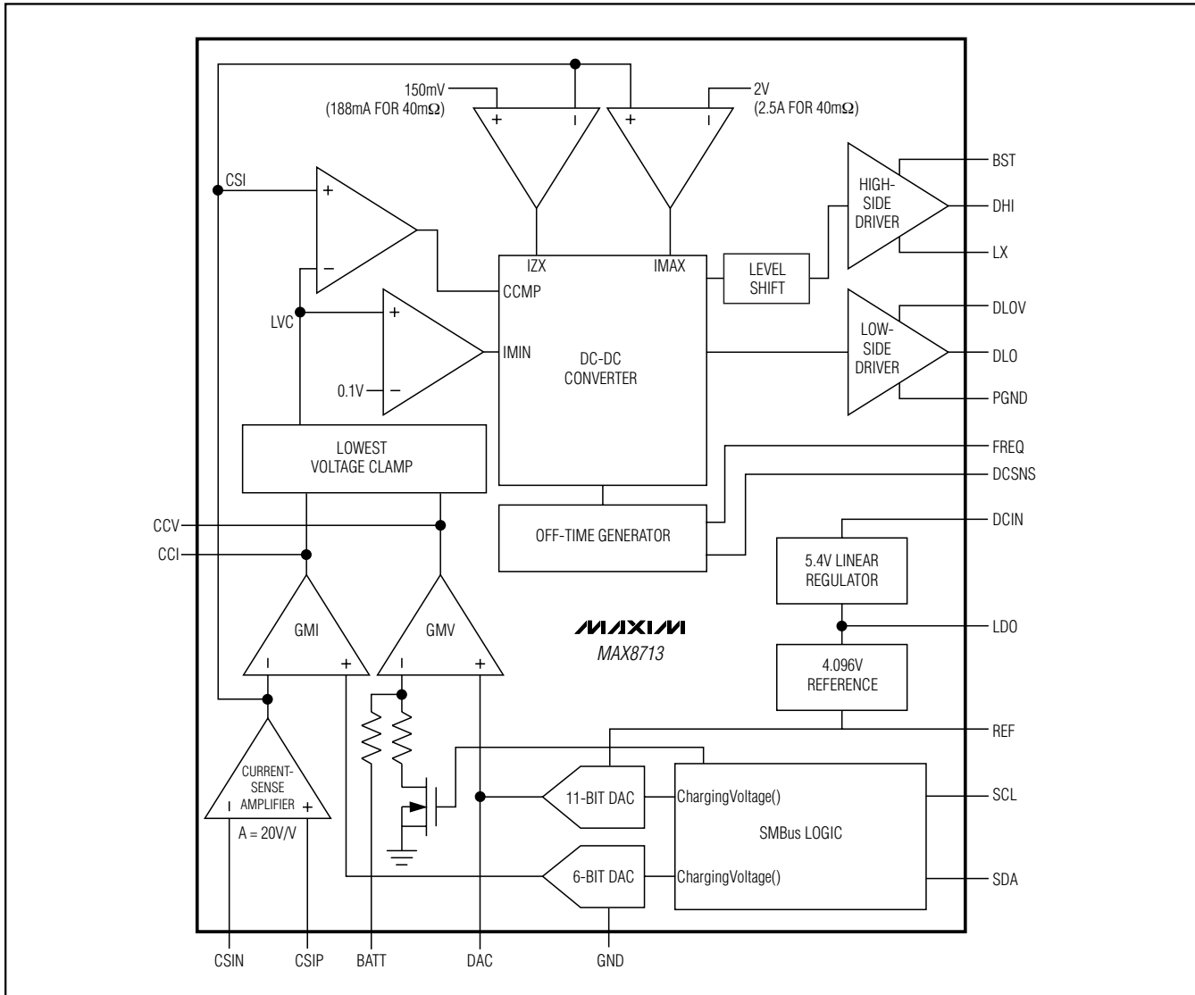
Figure 2. Functional Diagram
