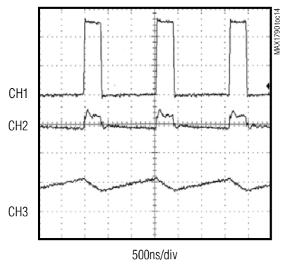
SWITCHING WAVEFORM
