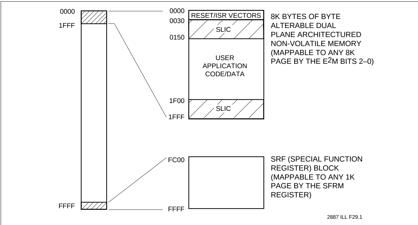
Figure 6. Microcontroller Map
