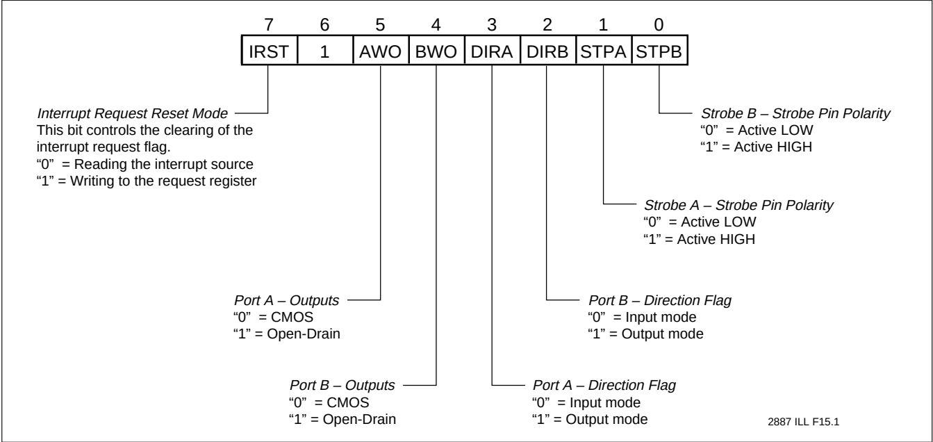
Figure 11. Configuration Register
