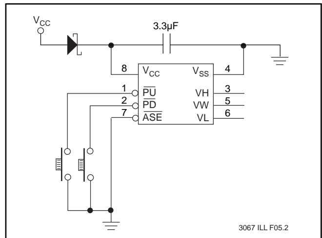
Typical circuit with \overline{ASE} store pin used in AUTOSTORE mode
