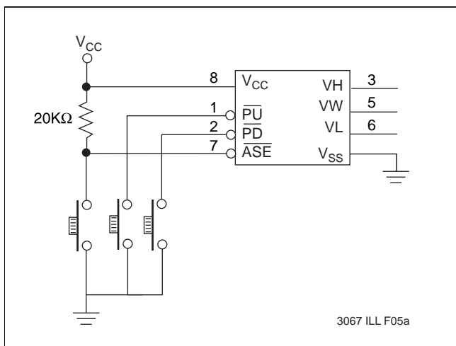
Typical circuit with \overline{ASE} store pin controlled by push button switch
