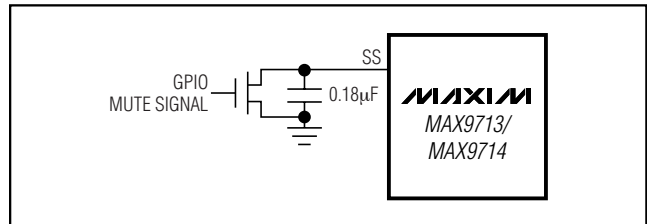
Figure 4. MAX9713/MAX9714 Mute Circuit
