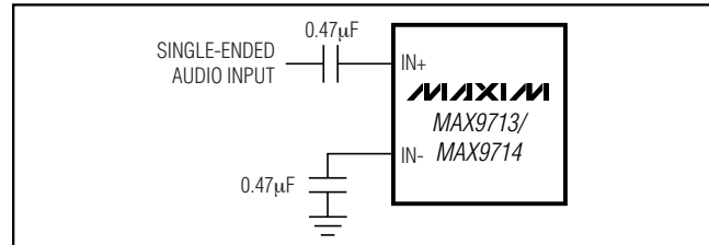
Figure 5. Single-Ended Input
