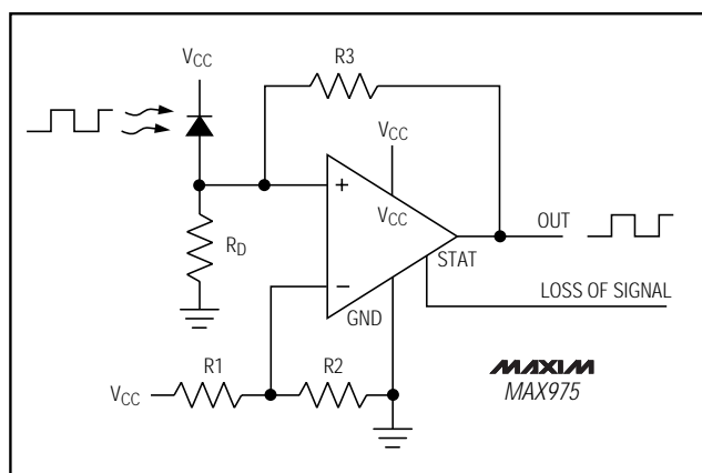
Figure 4. IR Receiver
