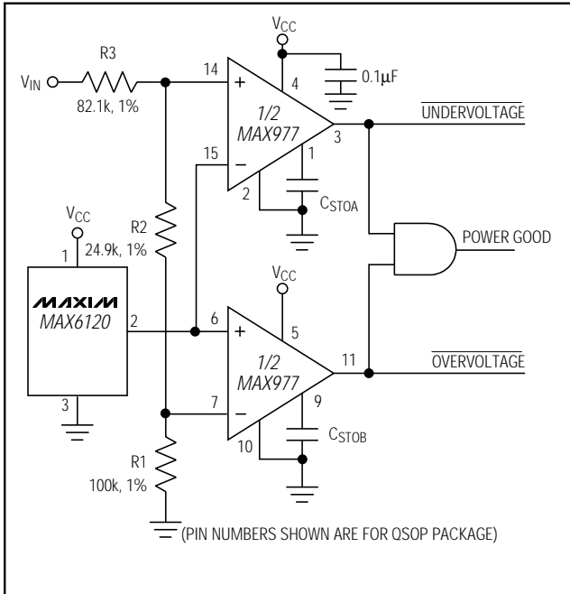
Figure 5. Window Comparator
