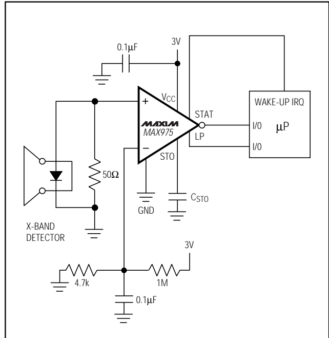
Figure 6. Toll-Tag Reader
