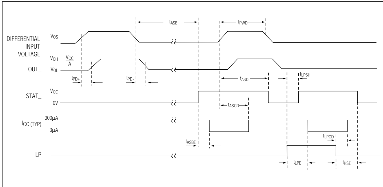
Figure 2. Timing Diagram
